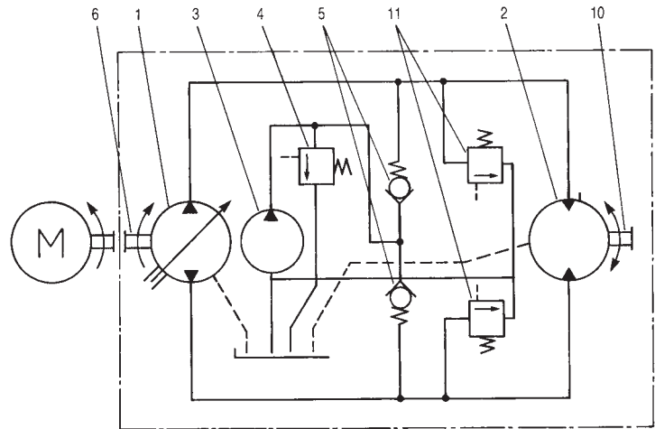
Hydraulic Schematic
